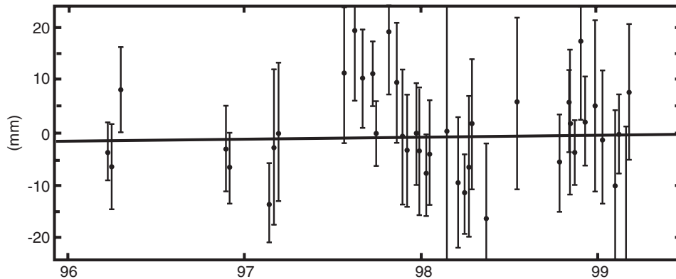
WES2 Up Offset rate(mm/yr) = 0.5 \pm 1.7
